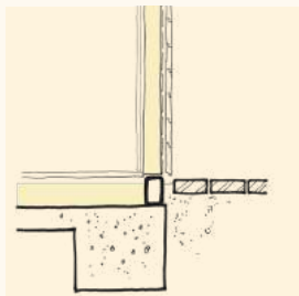
1999: Structure below ground requires additional protection
