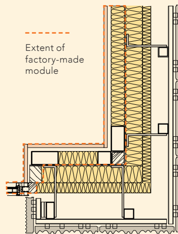
Mapleton Crescent: detail of wall build construction.
