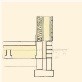
2019: Key interface between panels and ground floor
