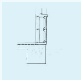
1940s: Defective! Lack of cover exposed steel reinforcement
