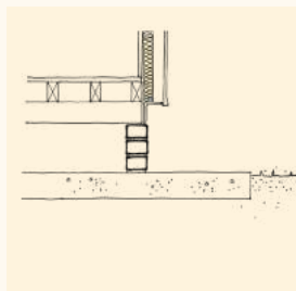
1944: Brick under-building protects metal structure
