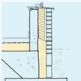
2018: Precast used as both structure and internal finish
