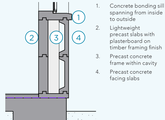
Orlit: Ground floor
